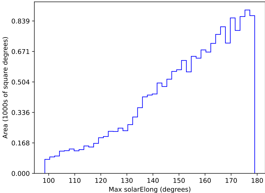
ddf_loaded_fl4_v3.4_10yrs WFD g band: Max solarElong
