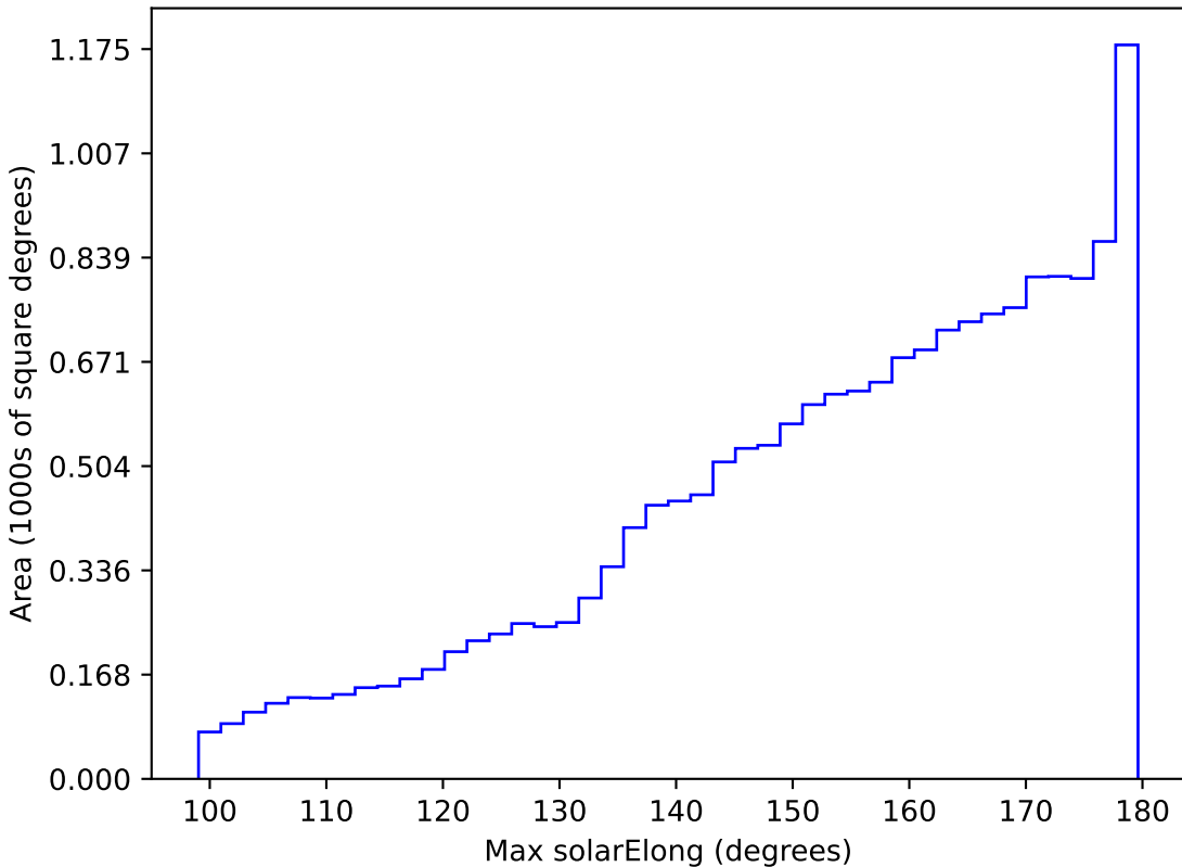
ddf_loaded_fl4_v3.4_10yrs WFD all bands: Max solarElong
