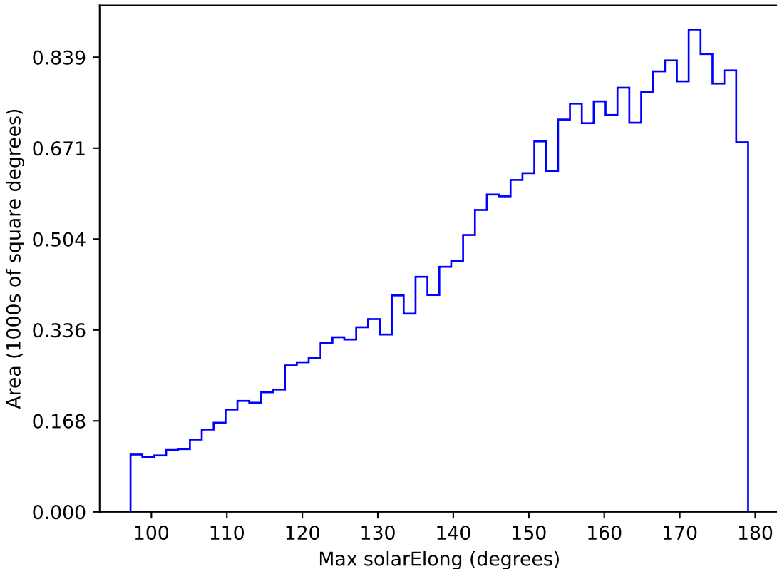
ddf_loaded_fl4_v3.4_10yrs All sky u band: Max solarElong
