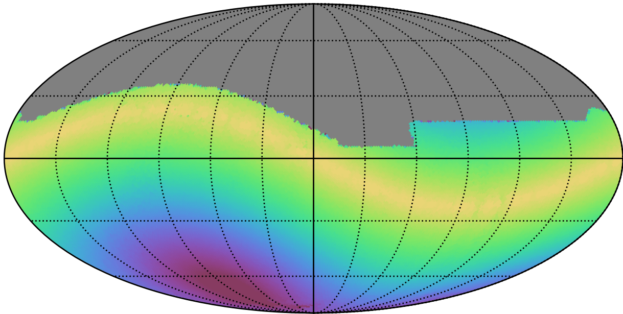
ddf_loaded_fl4_v3.4_10yrs All sky r band: Max solarElong
