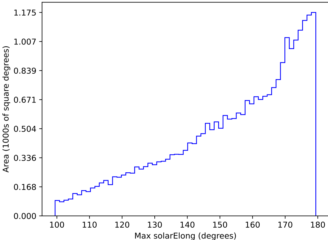
ddf_loaded_fl4_v3.4_10yrs All sky r band: Max solarElong
