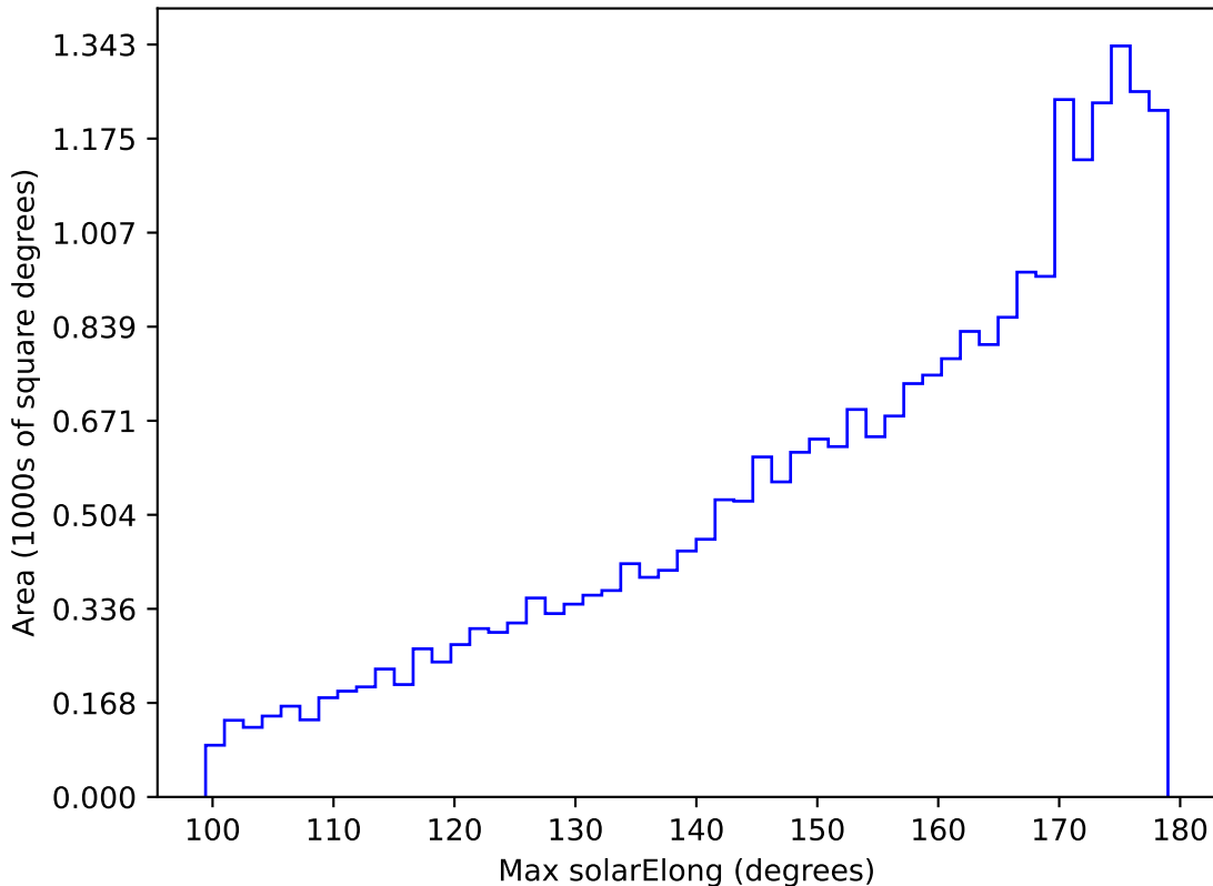
ddf_loaded_fl4_v3.4_10yrs All sky g band: Max solarElong
