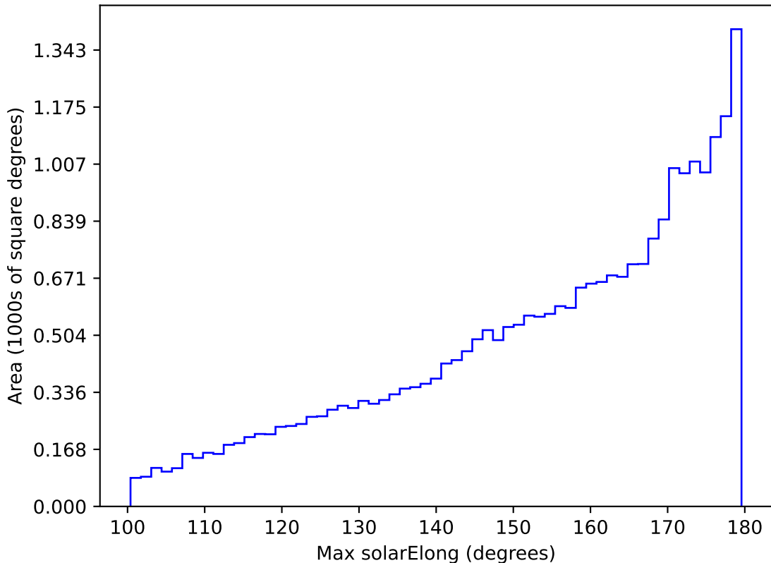
ddf_loaded_fl4_v3.4_10yrs All sky all bands: Max solarElong
