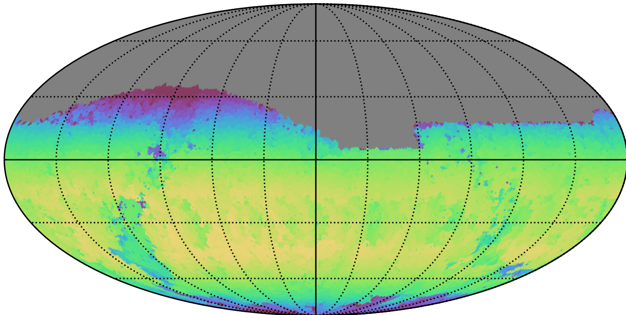
ddf_loaded_fl4_v3.4_10yrs Yr 1 z band: Max skyBrightness
