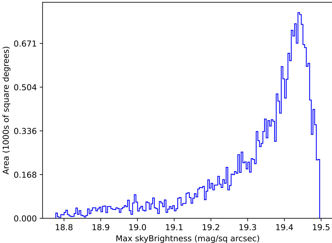
ddf_loaded_fl4_v3.4_10yrs Yr 1 z band: Max skyBrightness
