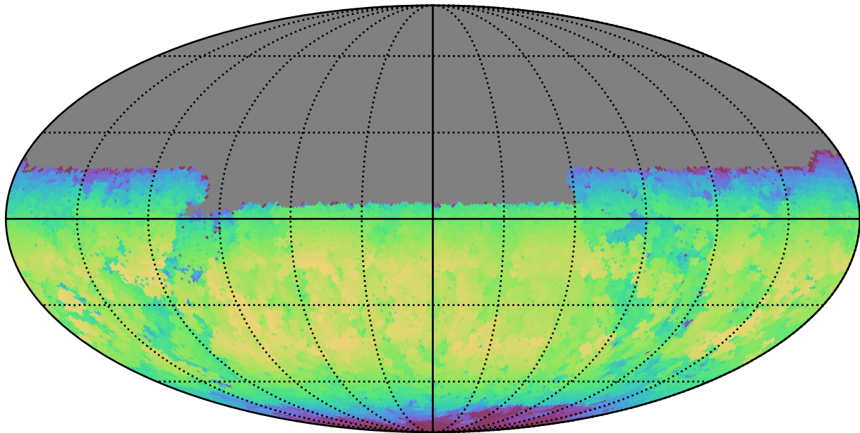
ddf_loaded_fl4_v3.4_10yrs Yr 1 y band: Max skyBrightness
