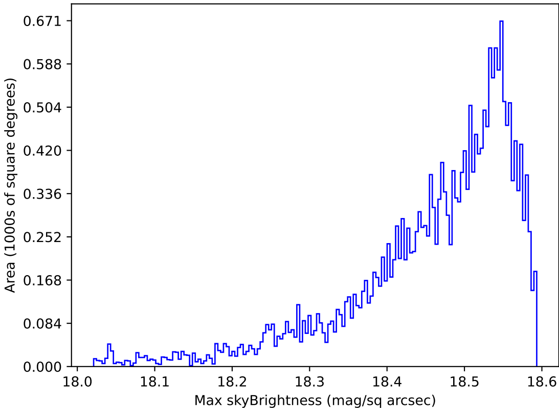
ddf_loaded_fl4_v3.4_10yrs Yr 1 y band: Max skyBrightness
