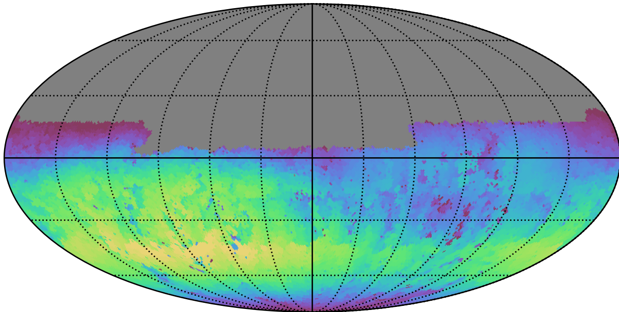
ddf_loaded_fl4_v3.4_10yrs Yr 1 u band: Max skyBrightness
