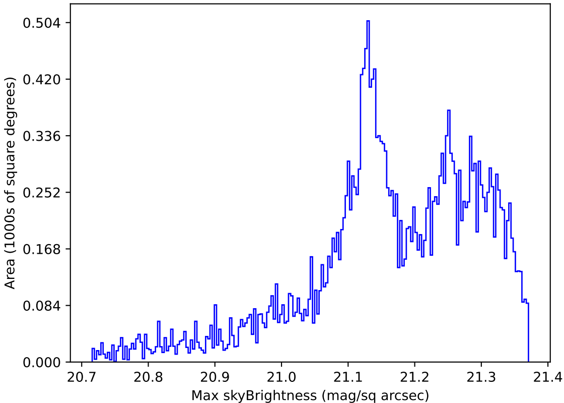
ddf_loaded_fl4_v3.4_10yrs Yr 1 r band: Max skyBrightness
