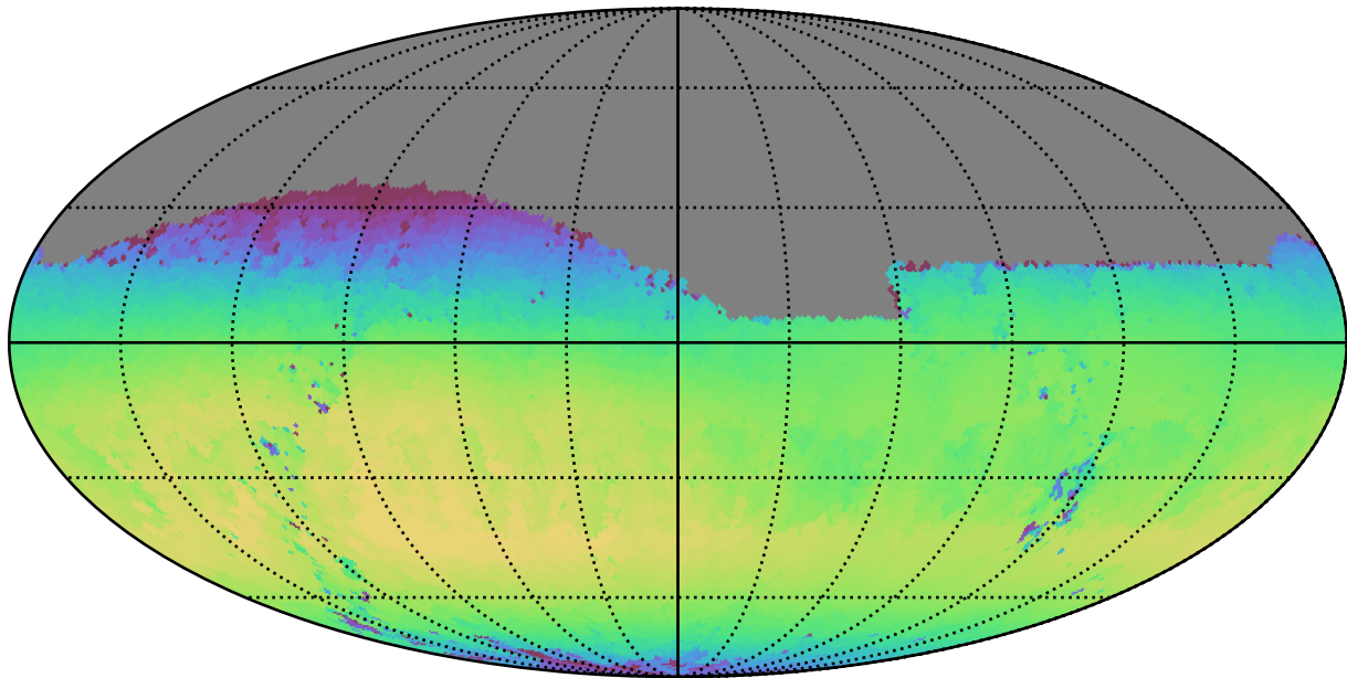
ddf_loaded_fl4_v3.4_10yrs Yr 1 i band: Max skyBrightness
