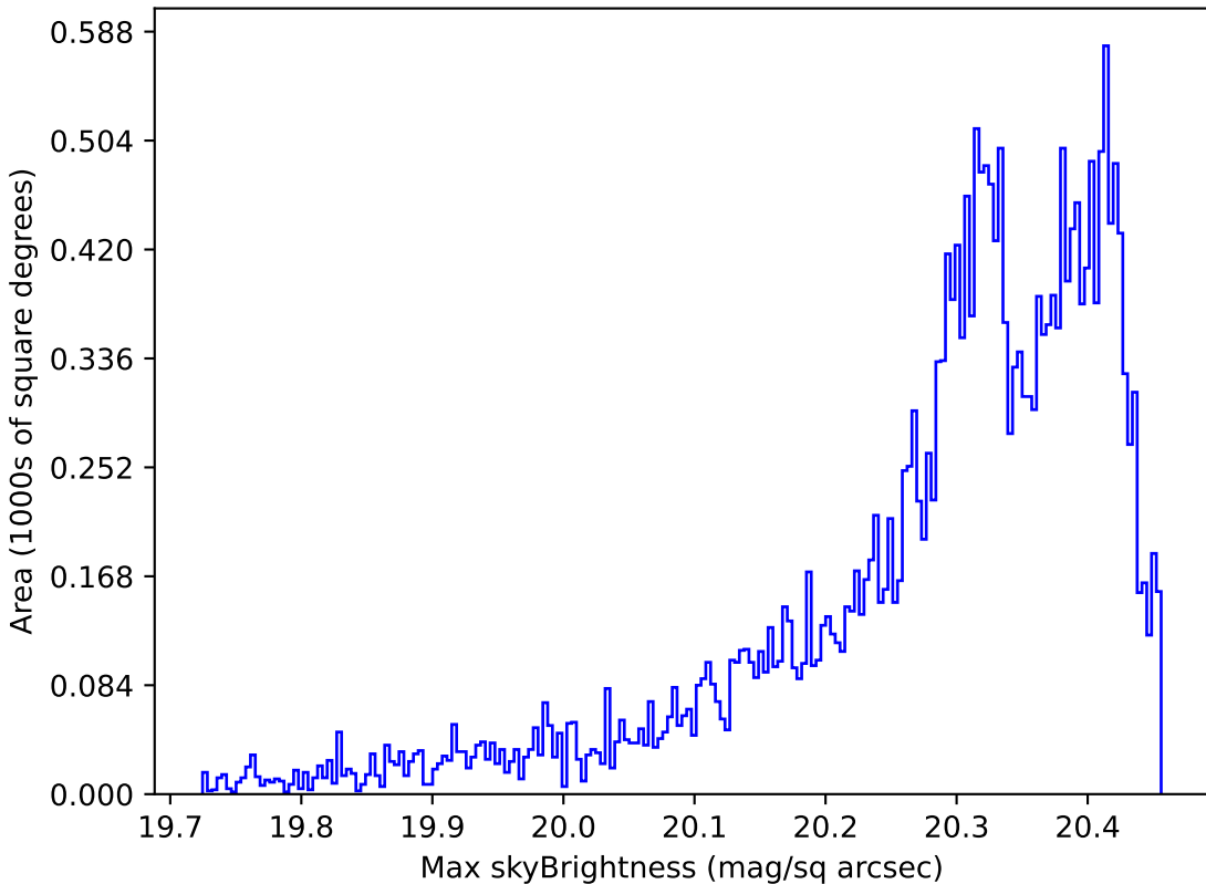
ddf_loaded_fl4_v3.4_10yrs Yr 1 i band: Max skyBrightness
