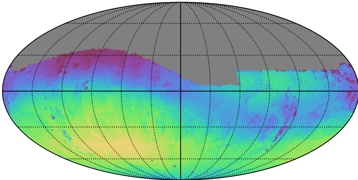
ddf_loaded_fl4_v3.4_10yrs Yr 1 g band: Max skyBrightness
