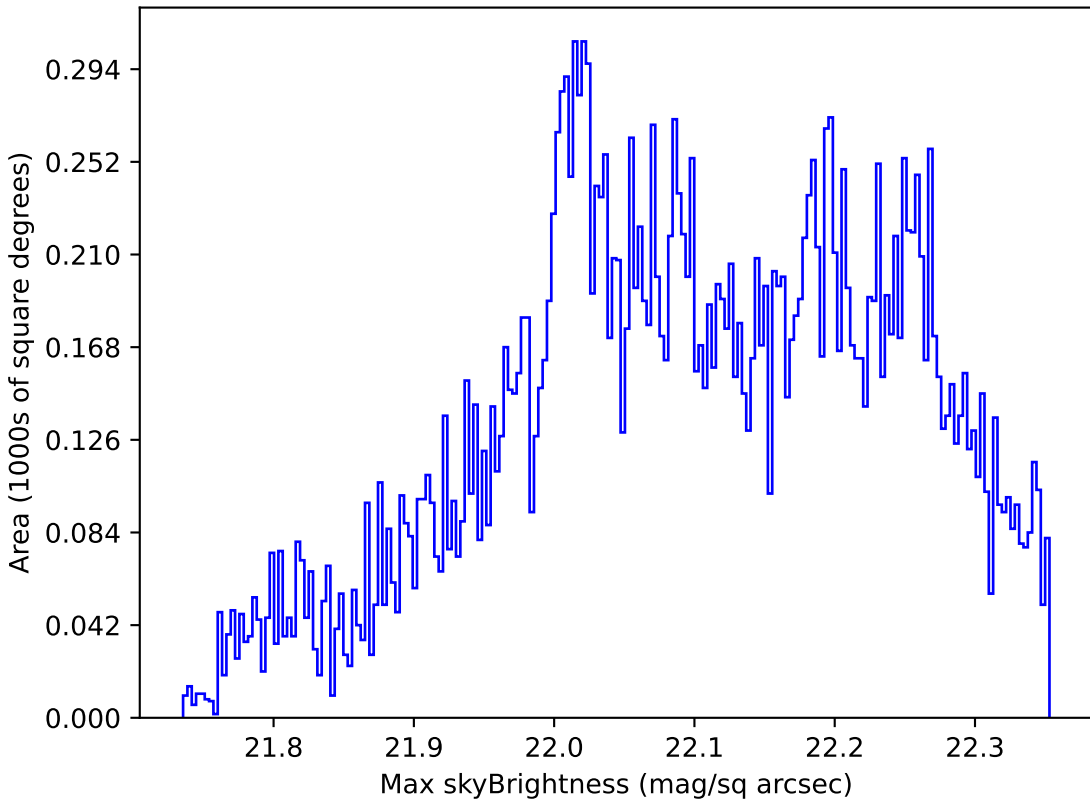
ddf_loaded_fl4_v3.4_10yrs Yr 1 g band: Max skyBrightness
