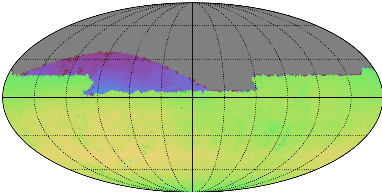
ddf_loaded_fl4_v3.4_10yrs Yr 1 all bands: Max skyBrightness
