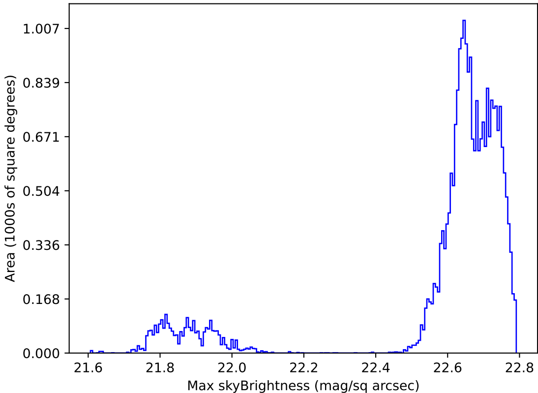
ddf_loaded_fl4_v3.4_10yrs Yr 1 all bands: Max skyBrightness
