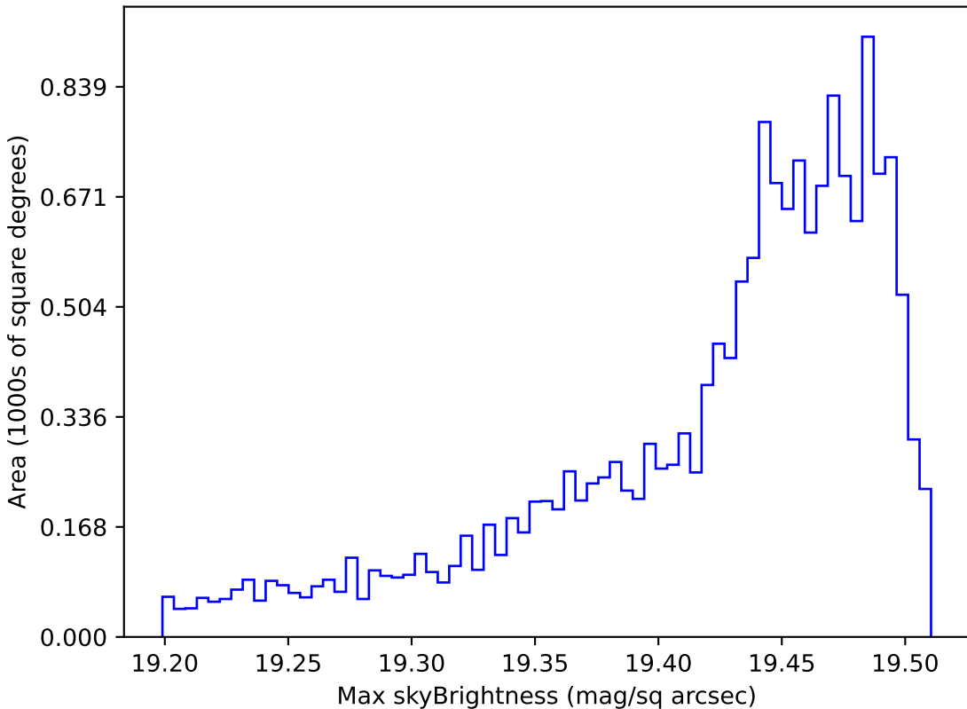
ddf_loaded_fl4_v3.4_10yrs WFD z band: Max skyBrightness
