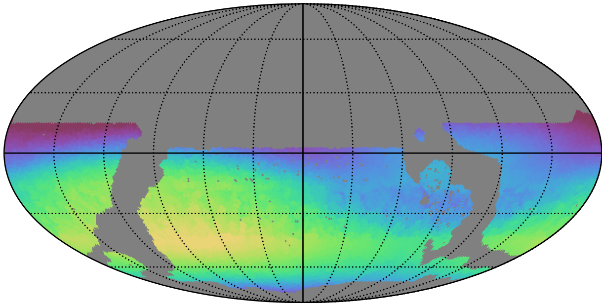
ddf_loaded_fl4_v3.4_10yrs WFD u band: Max skyBrightness
