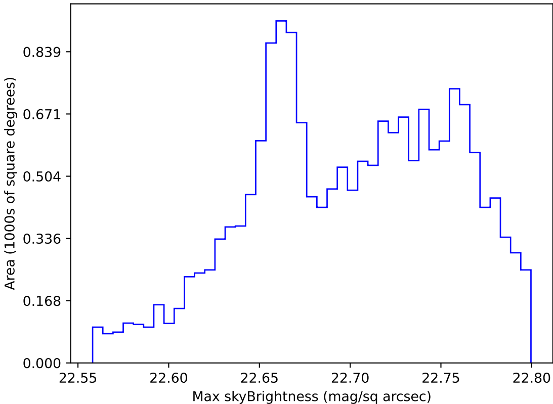
ddf_loaded_fl4_v3.4_10yrs WFD u band: Max skyBrightness
