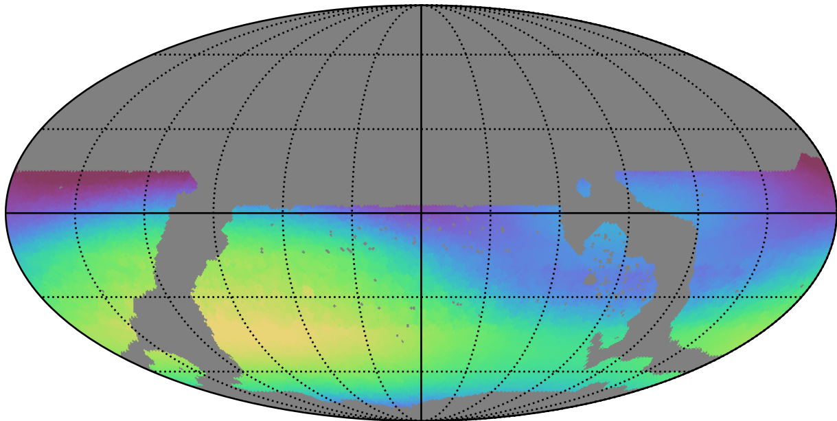
ddf_loaded_fl4_v3.4_10yrs WFD r band: Max skyBrightness
