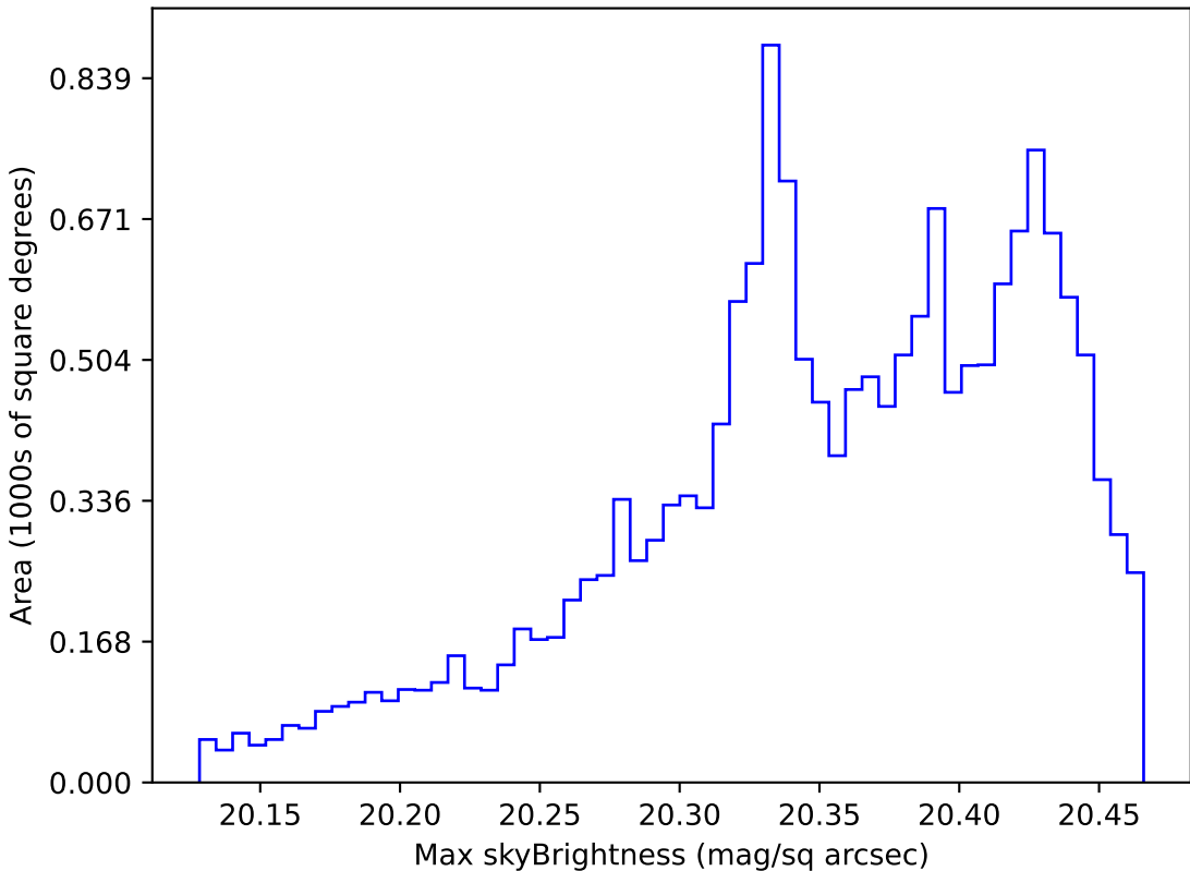
ddf_loaded_fl4_v3.4_10yrs WFD i band: Max skyBrightness
