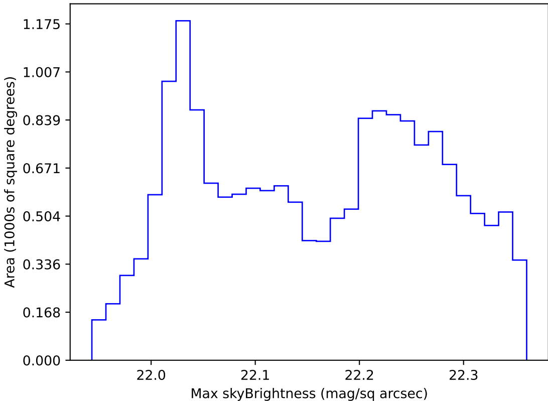
ddf_loaded_fl4_v3.4_10yrs WFD g band: Max skyBrightness
