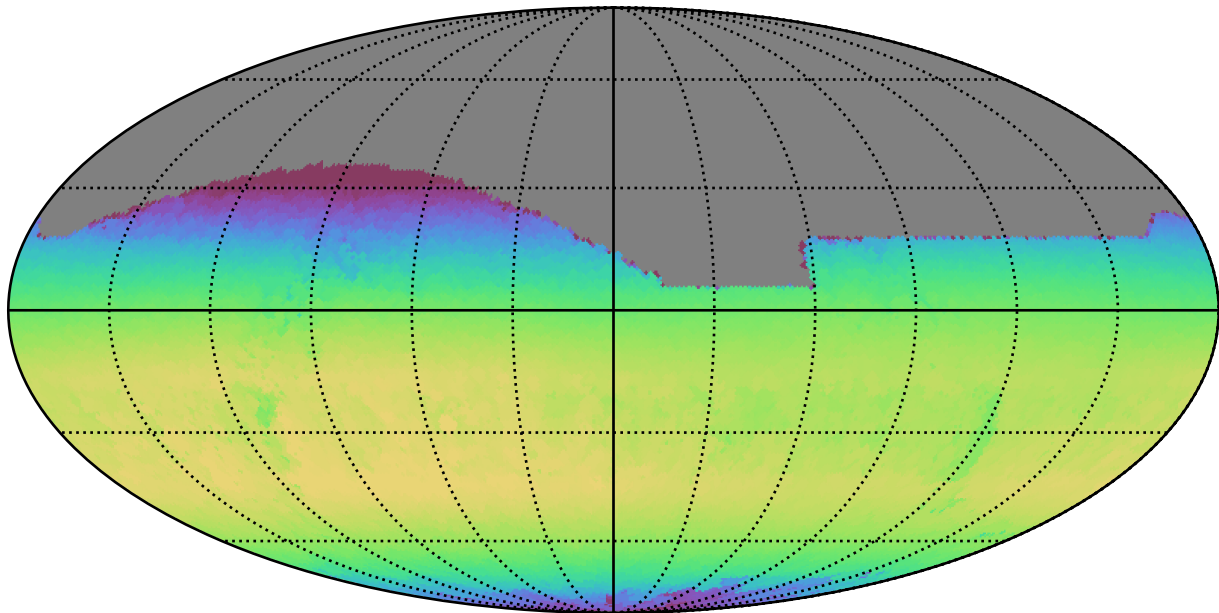
ddf_loaded_fl4_v3.4_10yrs All sky z band: Max skyBrightness
