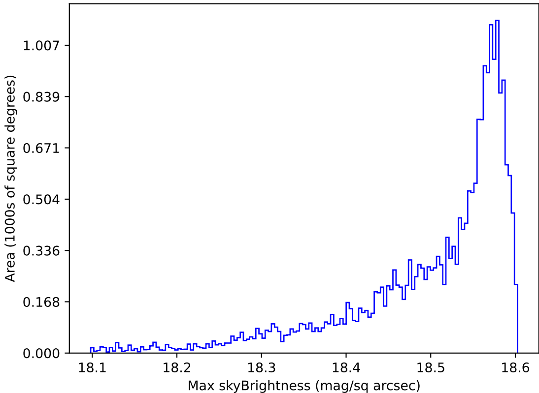
ddf_loaded_fl4_v3.4_10yrs All sky y band: Max skyBrightness
