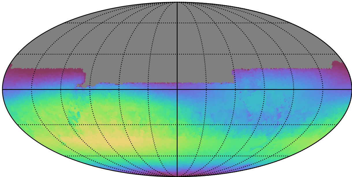
ddf_loaded_fl4_v3.4_10yrs All sky u band: Max skyBrightness
