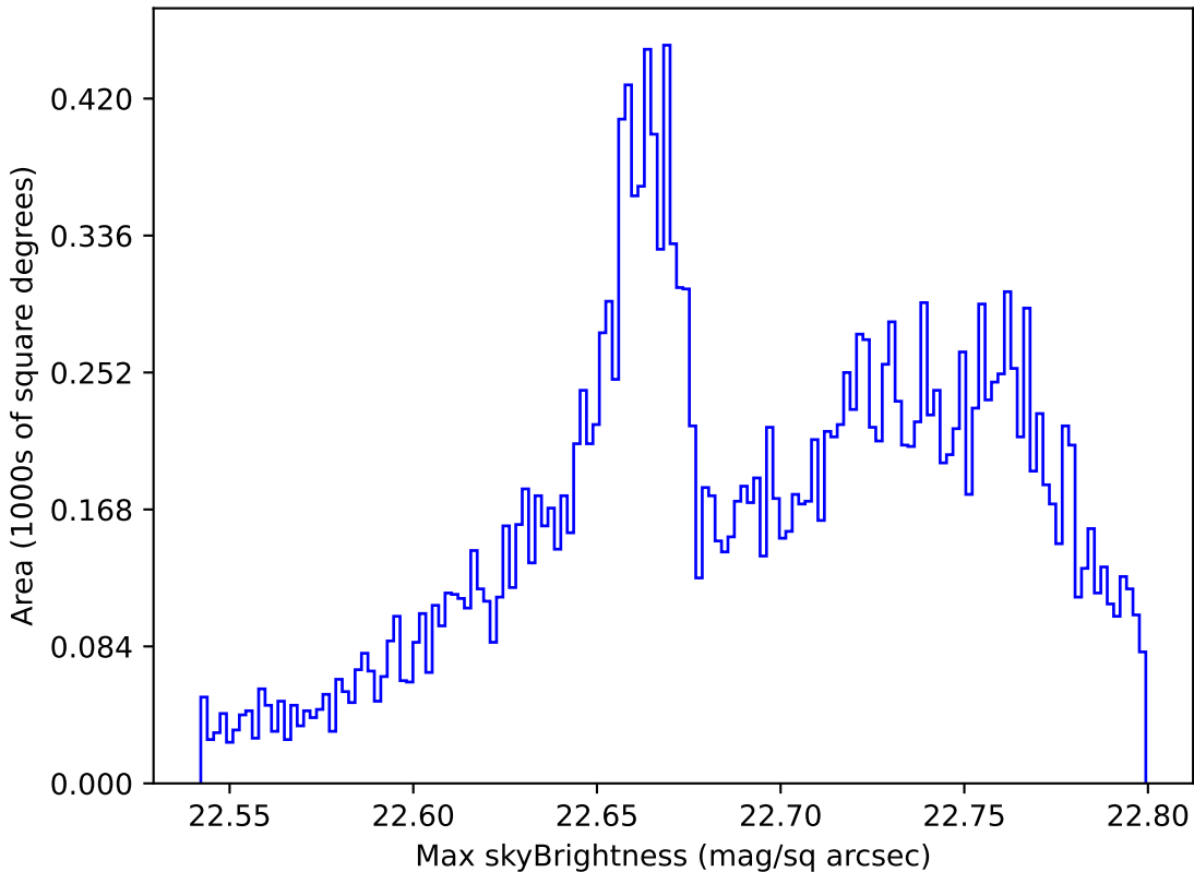
ddf_loaded_fl4_v3.4_10yrs All sky u band: Max skyBrightness
