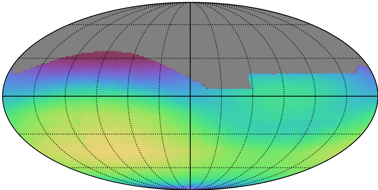
ddf_loaded_fl4_v3.4_10yrs All sky r band: Max skyBrightness
