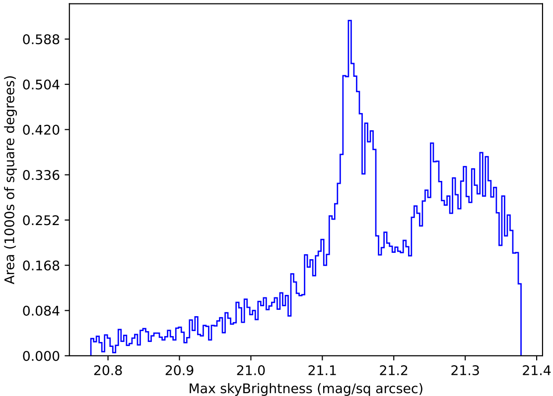
ddf_loaded_fl4_v3.4_10yrs All sky r band: Max skyBrightness
