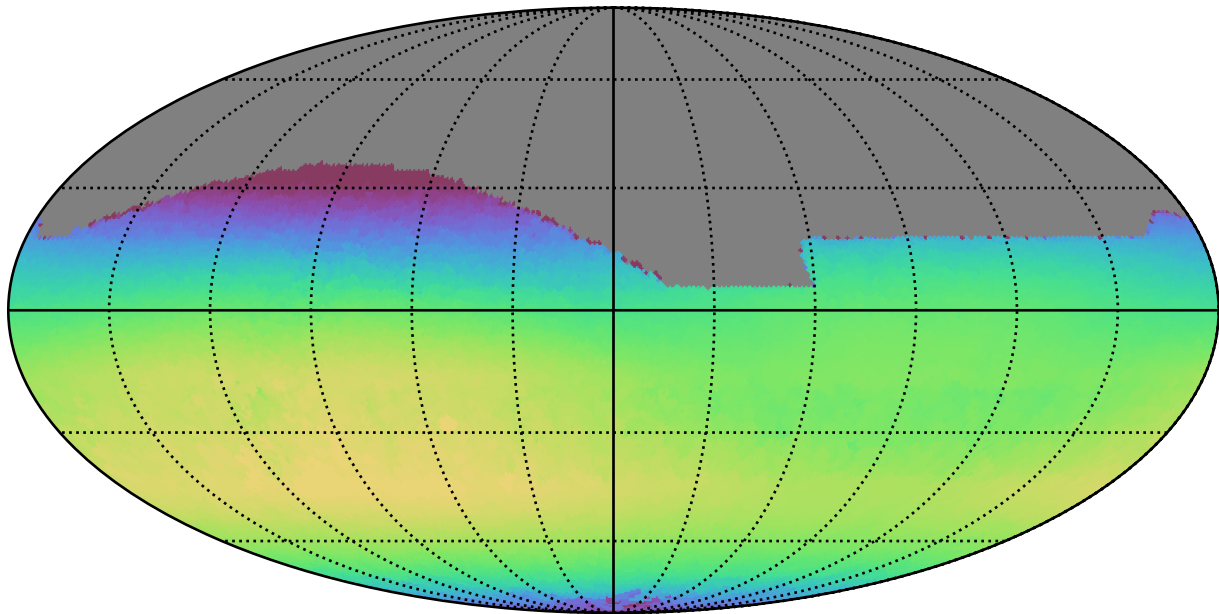
ddf_loaded_fl4_v3.4_10yrs All sky i band: Max skyBrightness
