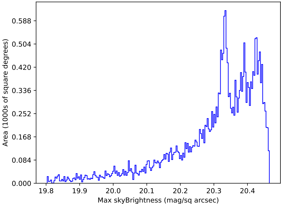
ddf_loaded_fl4_v3.4_10yrs All sky i band: Max skyBrightness
