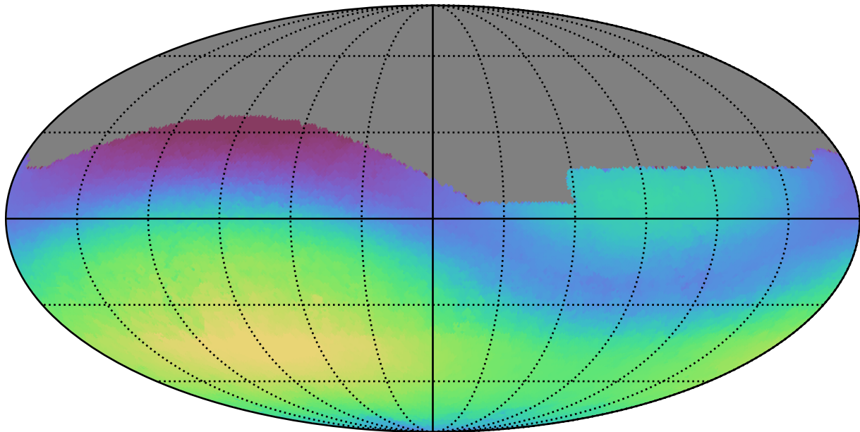
ddf_loaded_fl4_v3.4_10yrs All sky g band: Max skyBrightness
