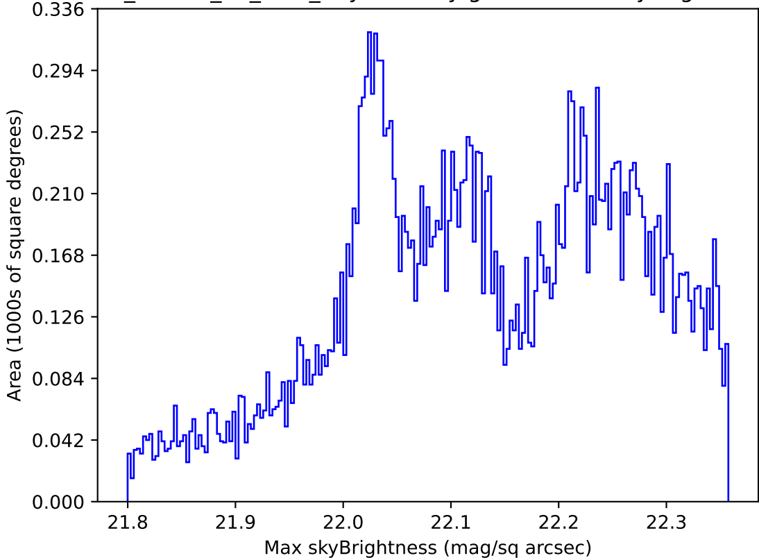
ddf_loaded_fl4_v3.4_10yrs All sky g band: Max skyBrightness
