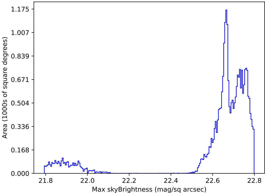
ddf_loaded_fl4_v3.4_10yrs All sky all bands: Max skyBrightness
