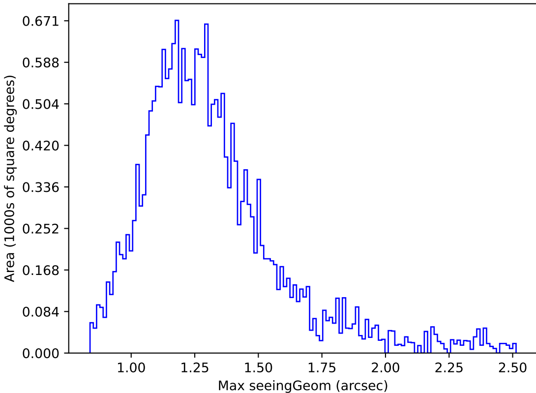
ddf_loaded_fl4_v3.4_10yrs Yr 1 y band: Max seeingGeom
