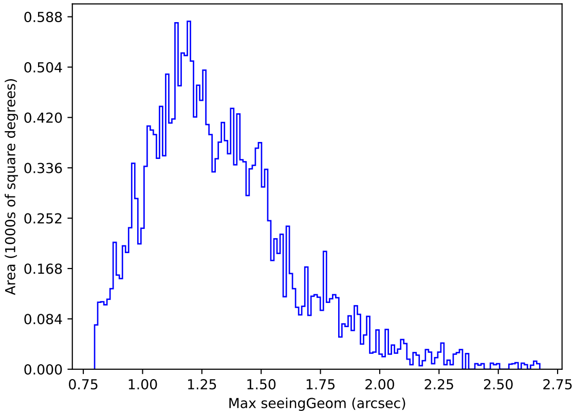
ddf_loaded_fl4_v3.4_10yrs Yr 1 u band: Max seeingGeom
