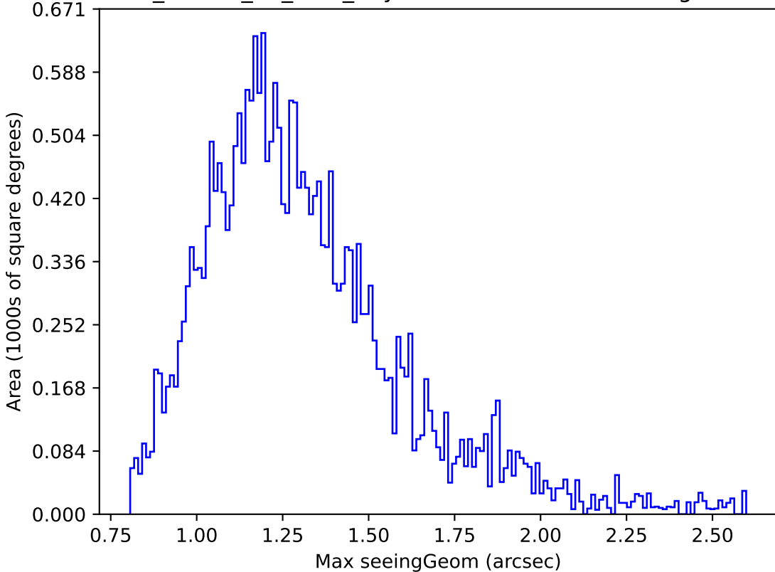
ddf_loaded_fl4_v3.4_10yrs Yr 1 i band: Max seeingGeom
