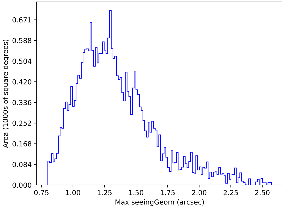
ddf_loaded_fl4_v3.4_10yrs Yr 1 g band: Max seeingGeom
