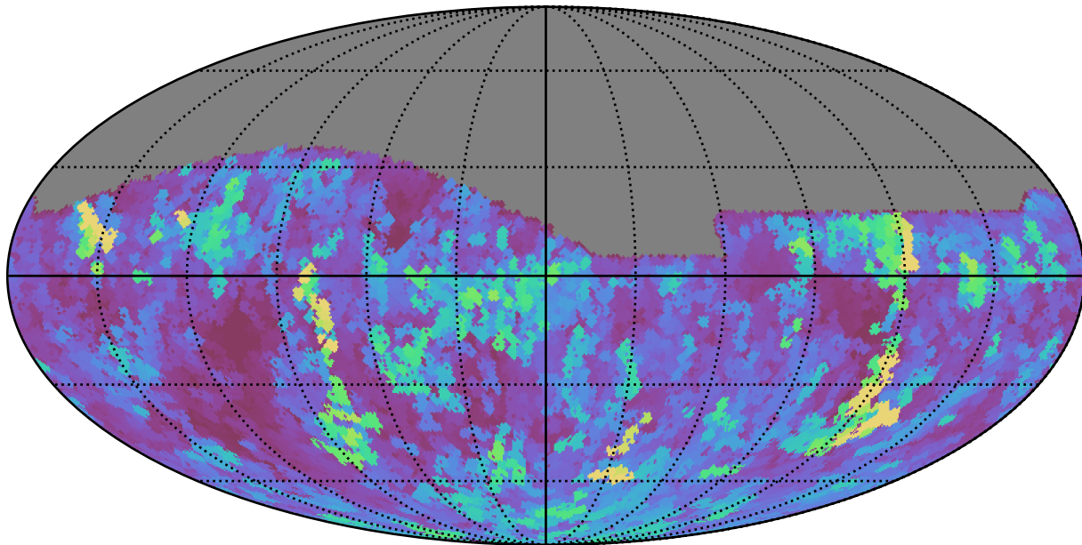
ddf_loaded_fl4_v3.4_10yrs Yr 1 all bands: Max seeingGeom
