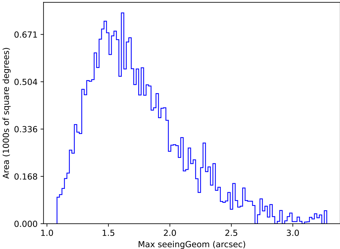
ddf_loaded_fl4_v3.4_10yrs Yr 1 all bands: Max seeingGeom
