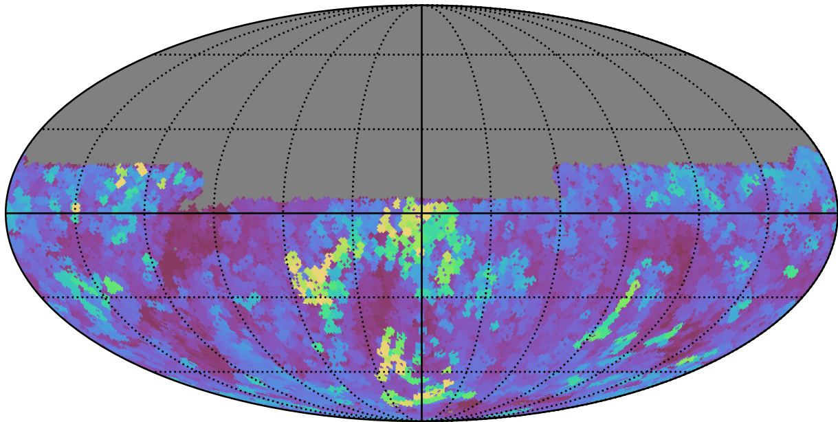
ddf_loaded_fl4_v3.4_10yrs Yr 1 y band: Max seeingEff
