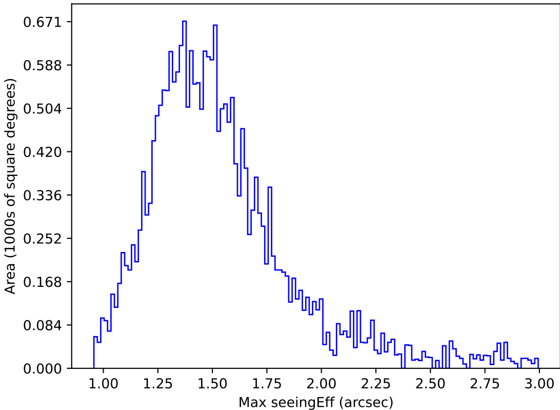
ddf_loaded_fl4_v3.4_10yrs Yr 1 y band: Max seeingEff
