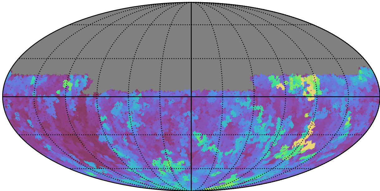
ddf_loaded_fl4_v3.4_10yrs Yr 1 u band: Max seeingEff
