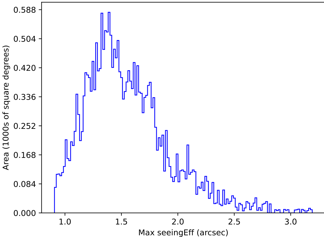
ddf_loaded_fl4_v3.4_10yrs Yr 1 u band: Max seeingEff
