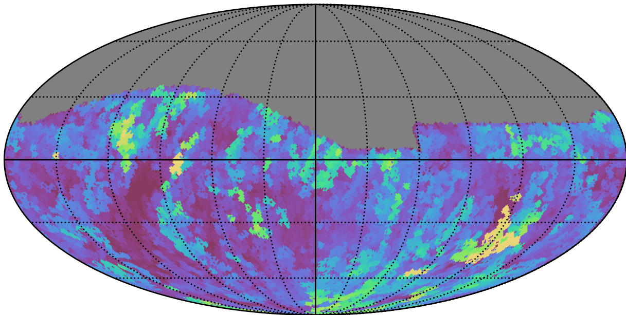
ddf_loaded_fl4_v3.4_10yrs Yr 1 r band: Max seeingEff
