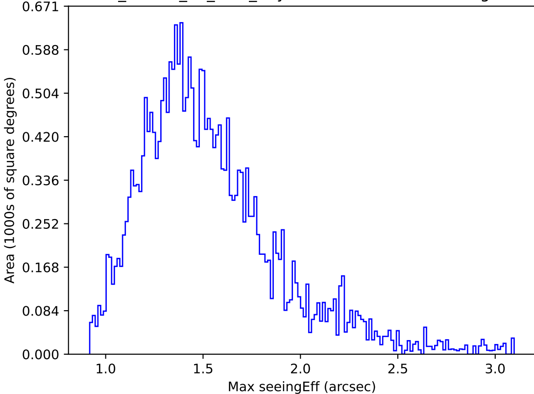
ddf_loaded_fl4_v3.4_10yrs Yr 1 i band: Max seeingEff
