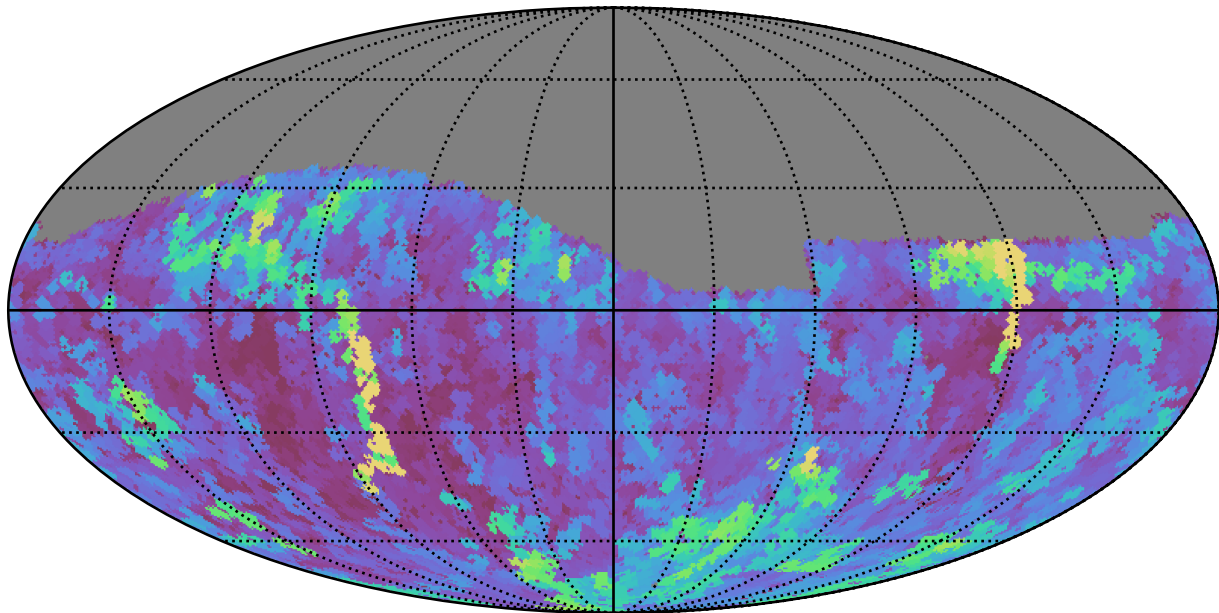
ddf_loaded_fl4_v3.4_10yrs Yr 1 g band: Max seeingEff
