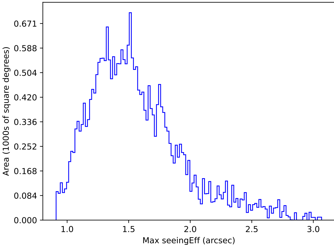
ddf_loaded_fl4_v3.4_10yrs Yr 1 g band: Max seeingEff
